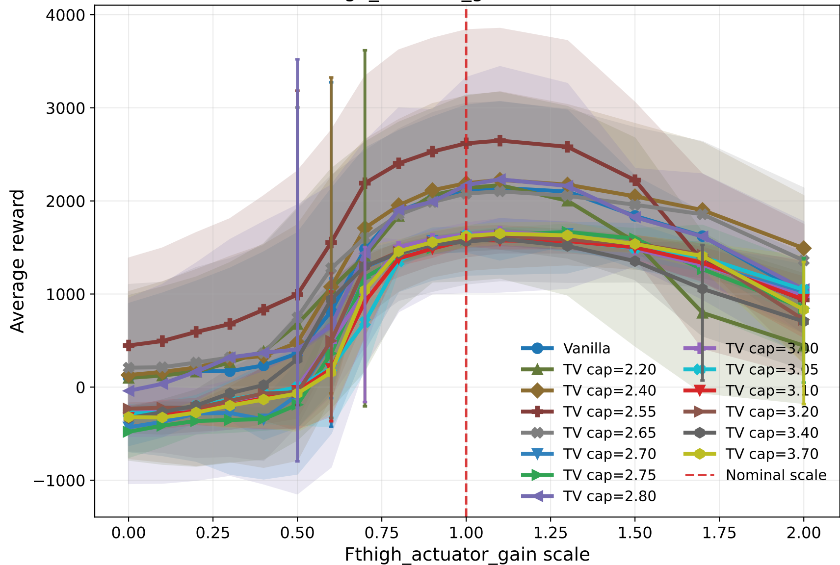
Fthigh actuator gain robustness
